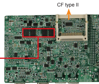
Solder Side
